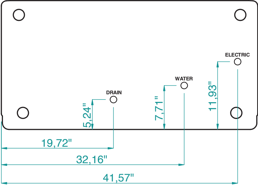
FRONT (BOTTOM VIEW)
